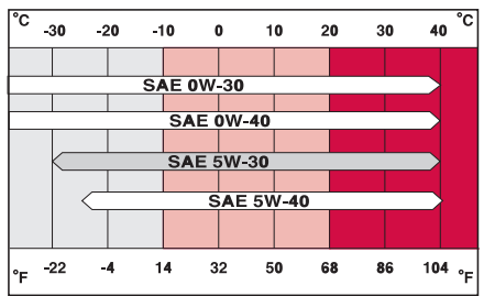
Viscosity chart
